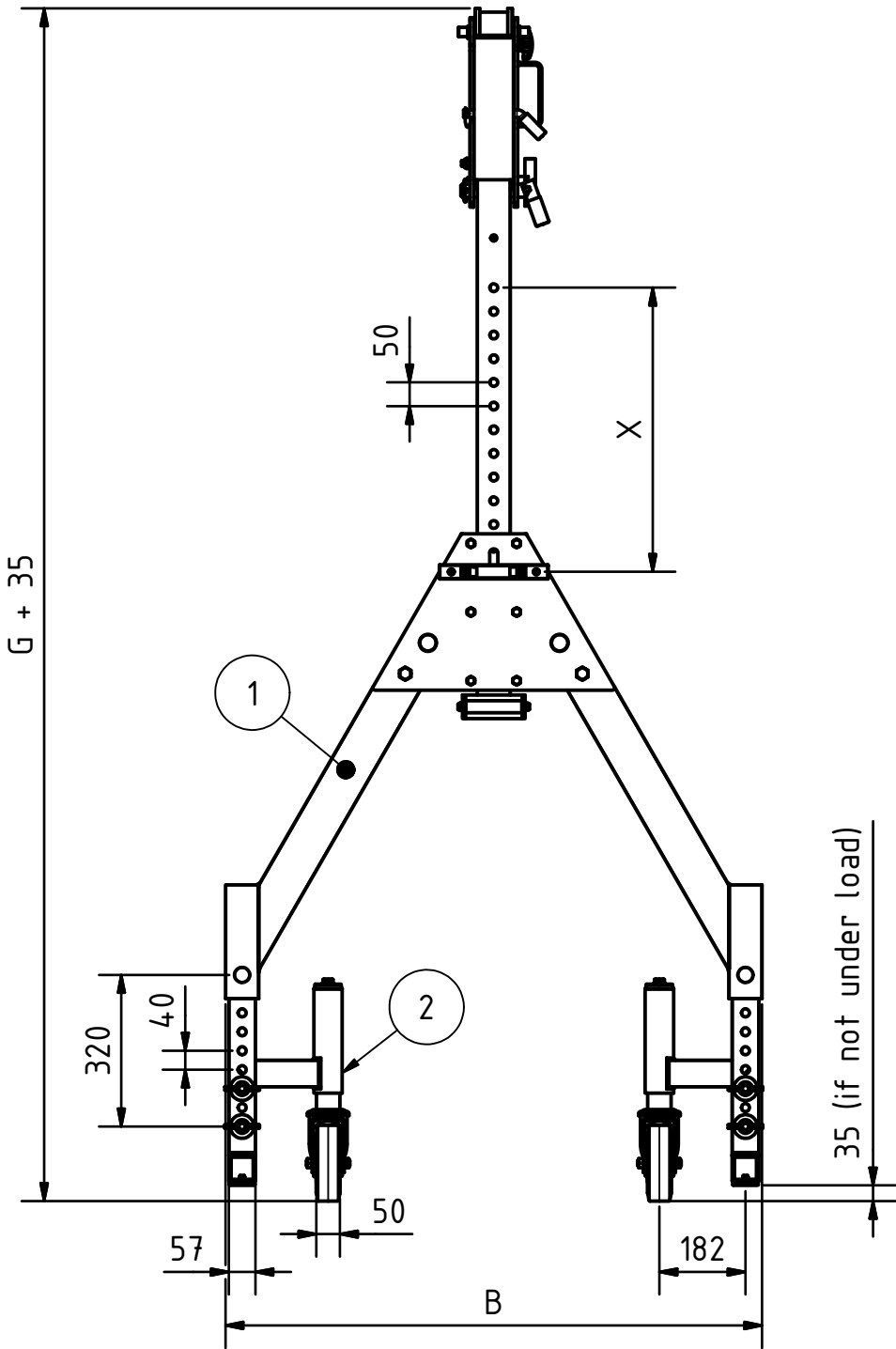
Fig. Crane Foldable Mini with 3m beam (111000-3) Dimensions in millimeters (mm)
