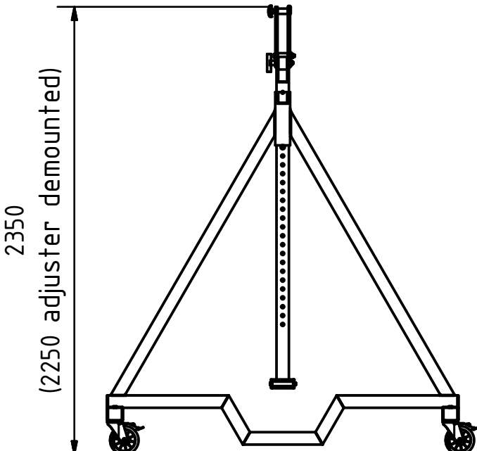
Side frame with adjuster
