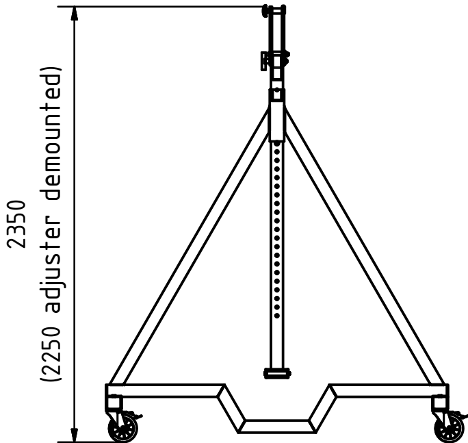
Side frame with adjuster
