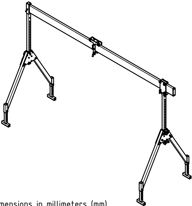
Dimensions in millimeters (mm)
