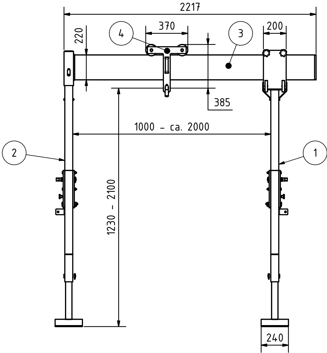
Side frame without adjuster folded
